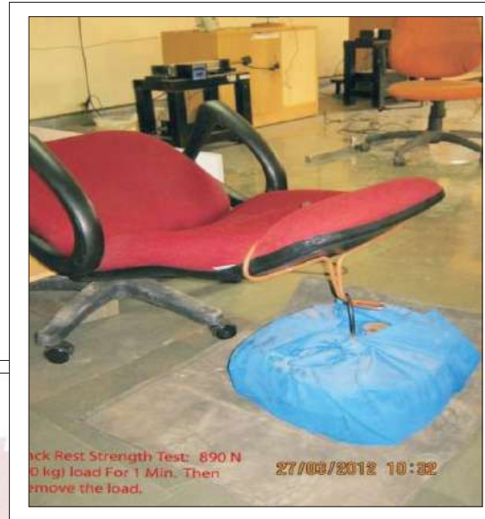
Back rest strength test
